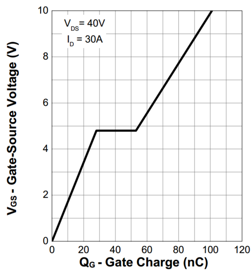
12. Gate Charge
