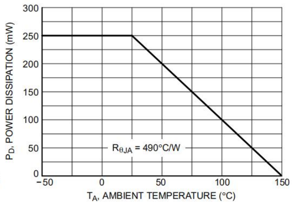
Figure 06. Derating Curve
