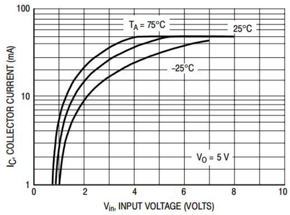
Figure 04. Output Current versus Input Voltage
